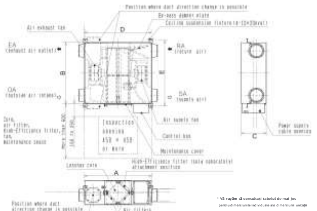
Dimensiuni LGH-25-100RVX-E *
