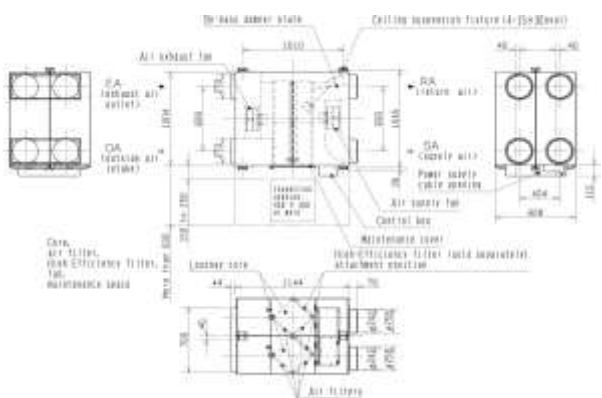
Dimensiuni LGH-150RVX-E
